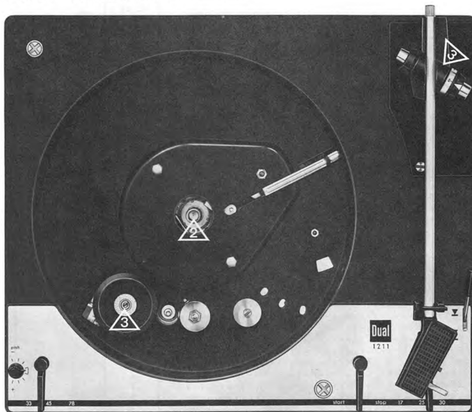
Fig. 24 Chassis, viewed from above
