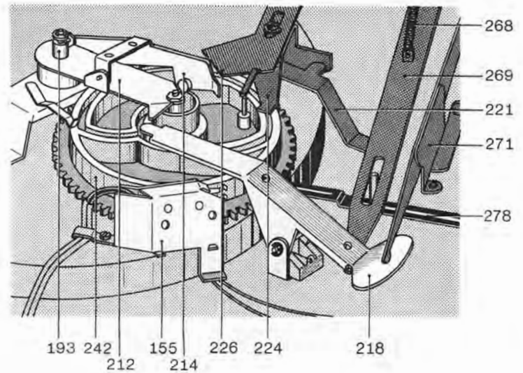
Fig. 15 Record drop
