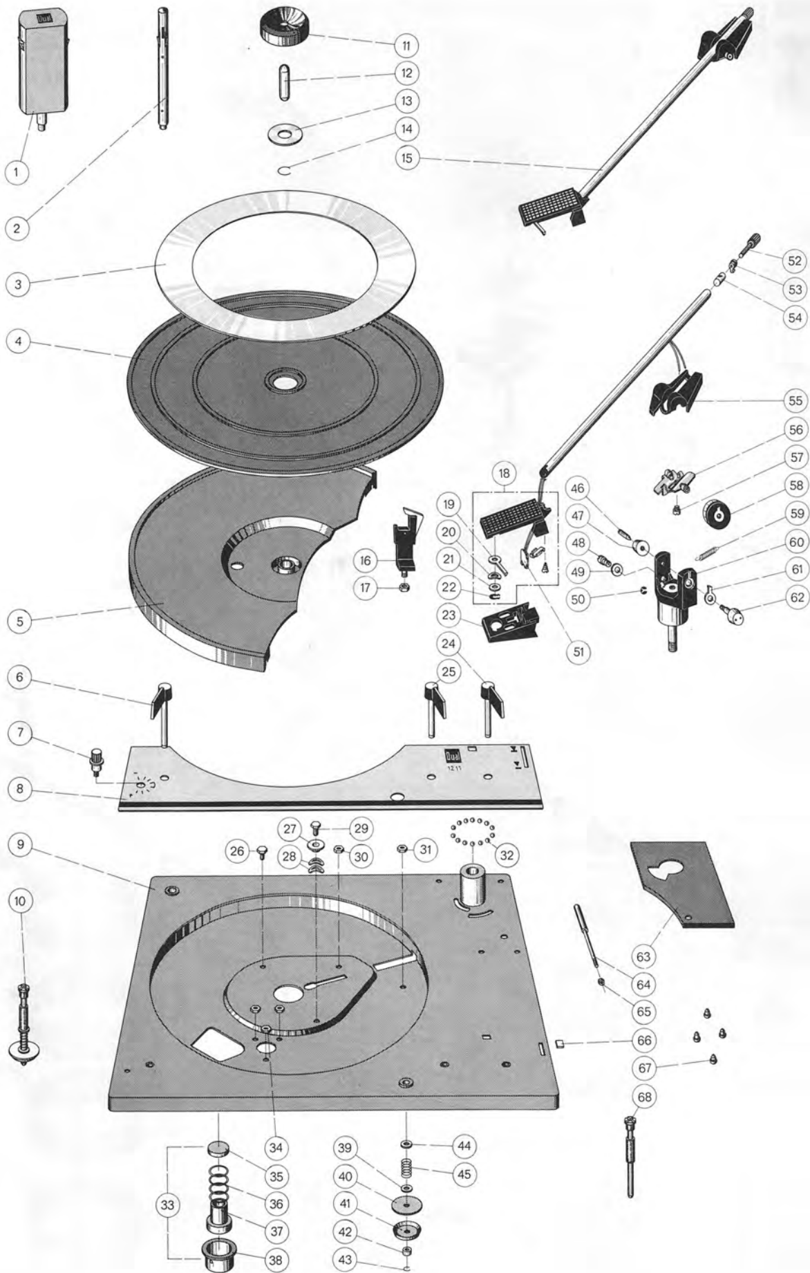
Fig. 26 Exploded view, parts above chassis
