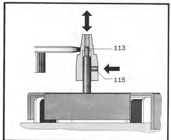
Fig. 6 Motor pulley position (4-pole motor)
