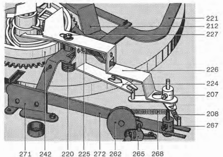
Fig. 12 Start position
