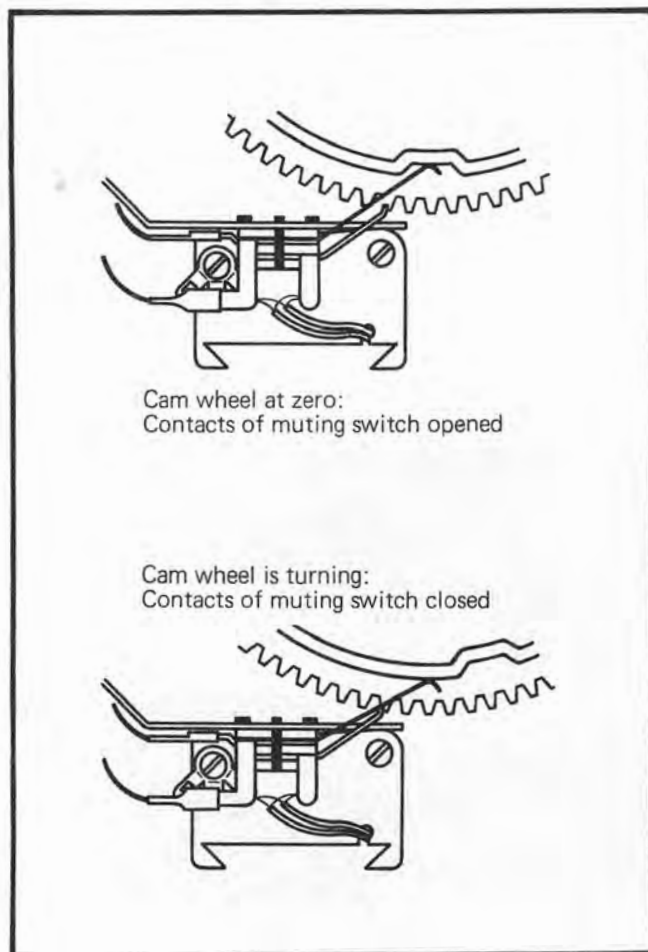
Fig. 14 Muting switch
