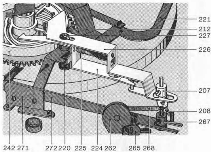
Fig. 13 Stop position
