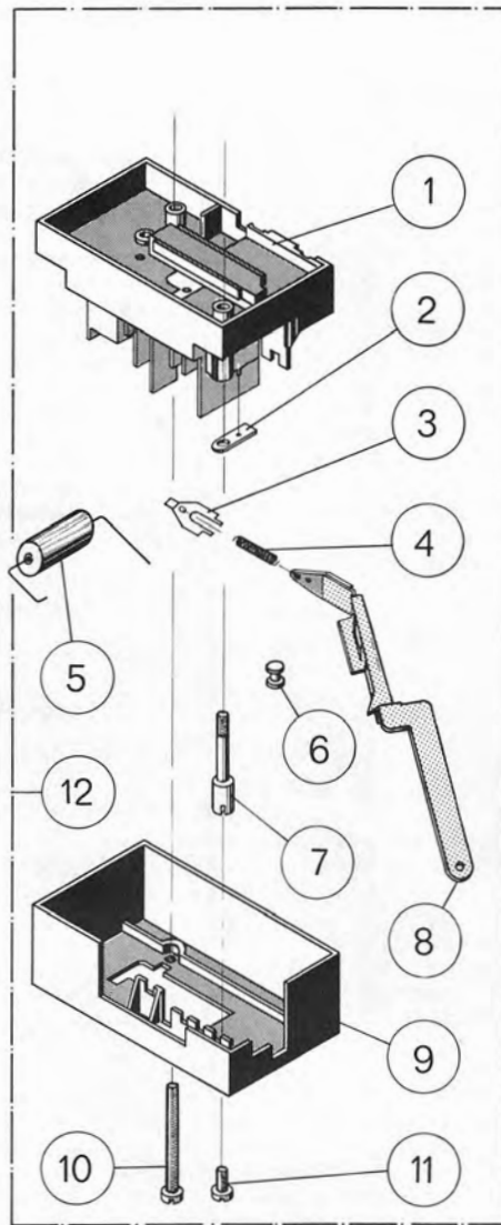
Fig. 28 Power switch (66,5 x 38,5 x 30,5) starting with Serial Number 186 459
