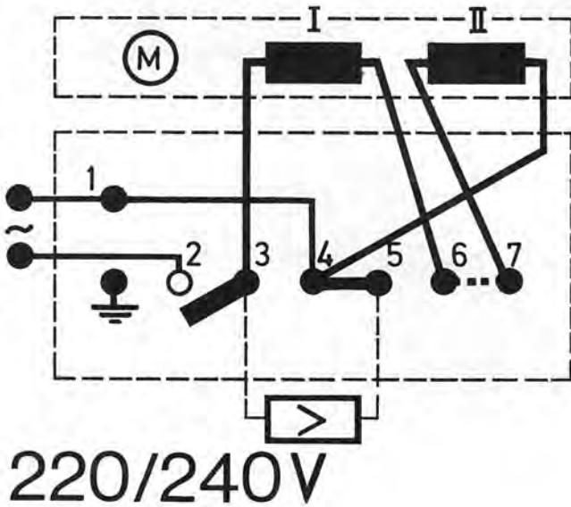
Fig. 4 Motor field connections (with voltage selector)
