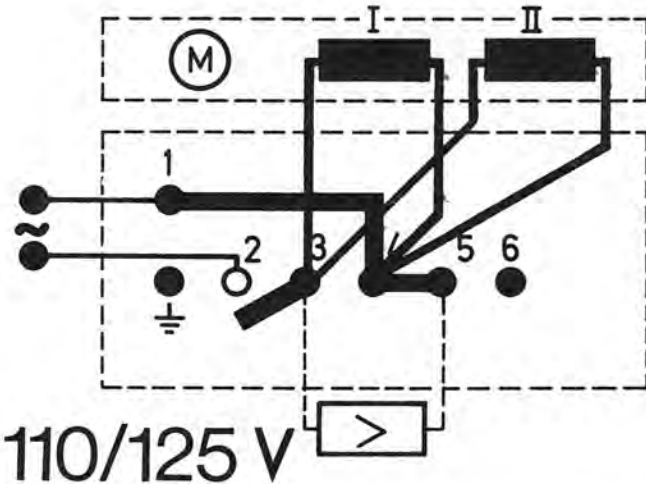
Fig. 3 Motor field connections (less voltage selector)
