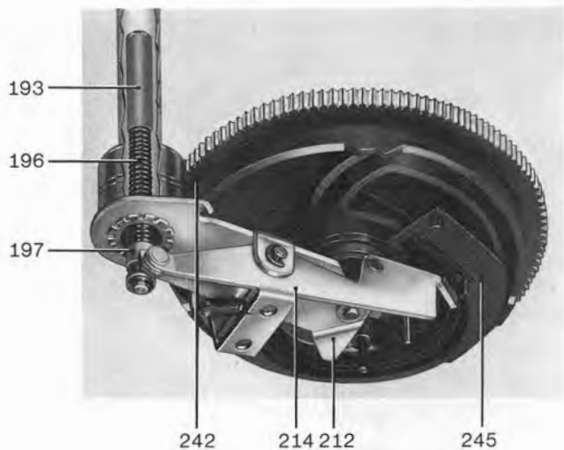
Fig. 17 Change cycle
