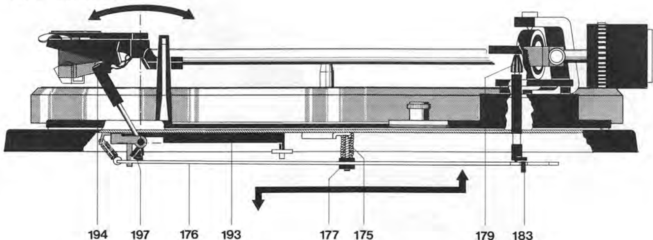
Fig. 8 Cue Control
