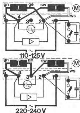
Fig. 4 Motor field coil connections
