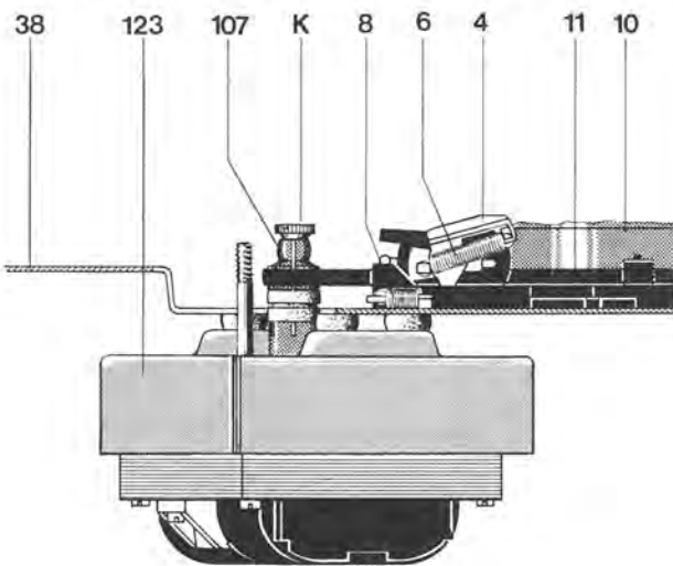
Fig. 2 Motor and Drive
