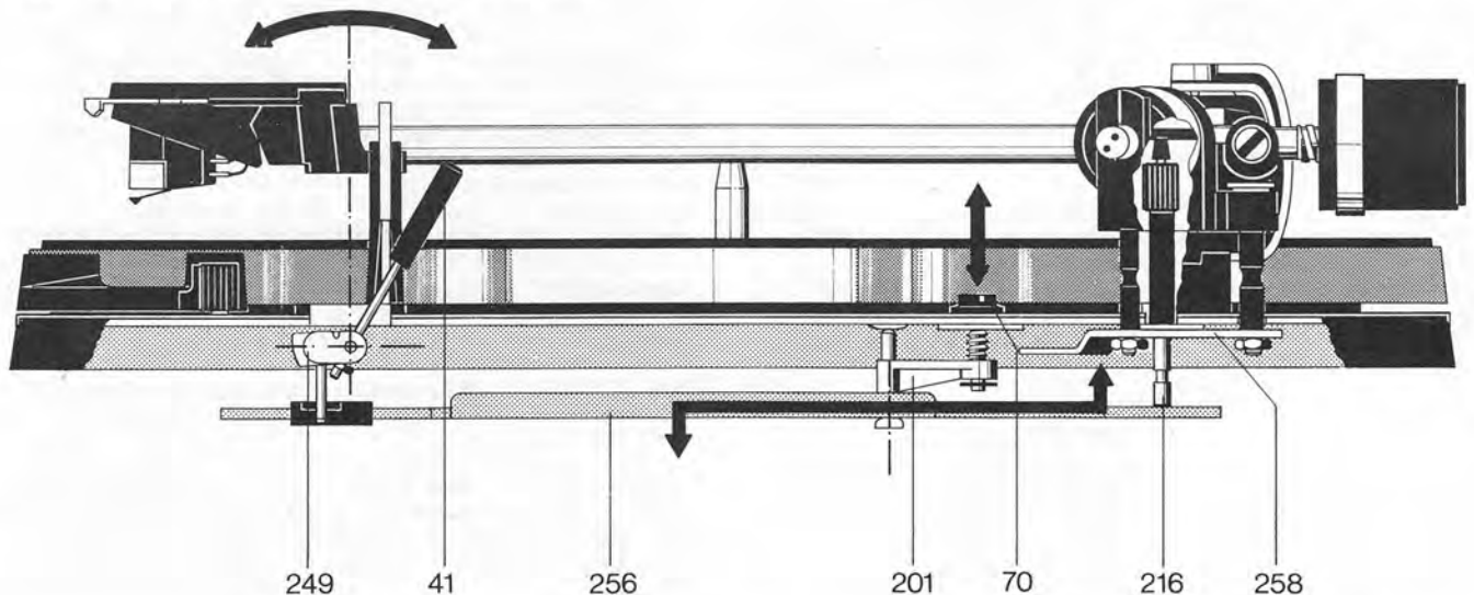
Fig. 15 Tonearm lift (tonearm raised)
