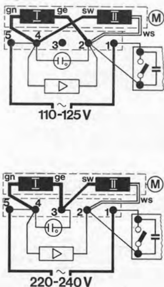
Fig. 7 Motor field connections (with voltage selector)
