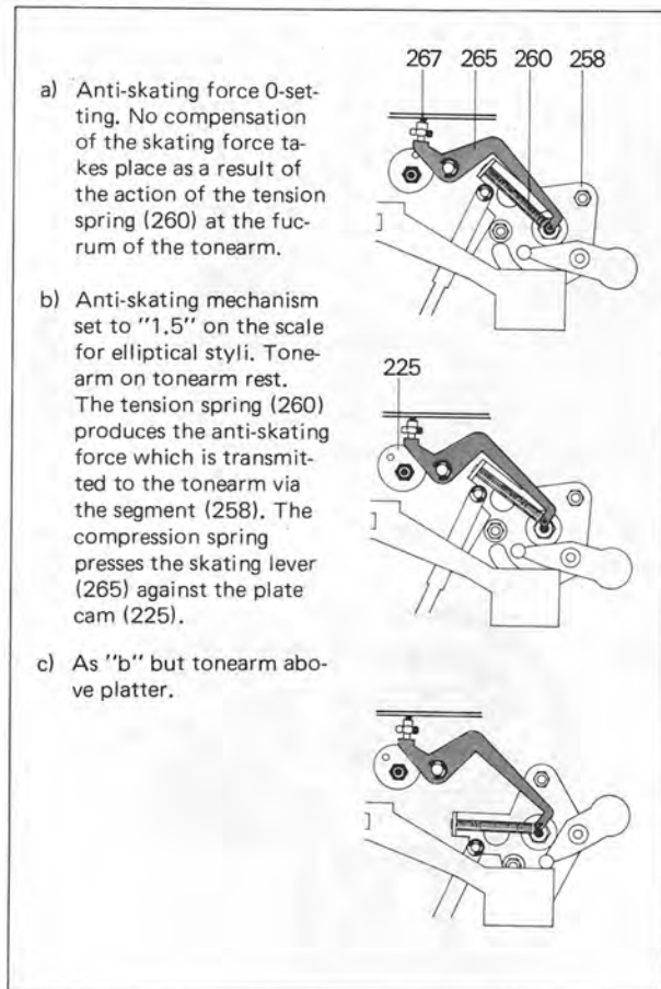
Fig. 13 Anti-skating force
