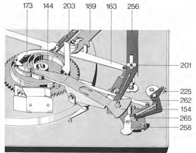
Fig. 14 Tonearm guide mechanism
