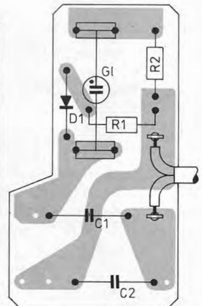
Circuit board (output stages)
