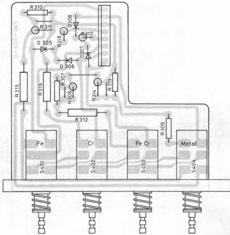
Tastenplatte / Push switch board / Plaque de touches 268 283
