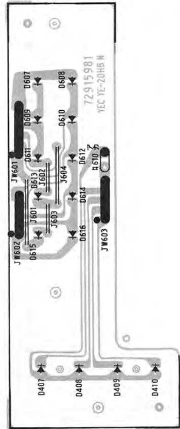
LED-platte / LED board / Plaque de LED L
